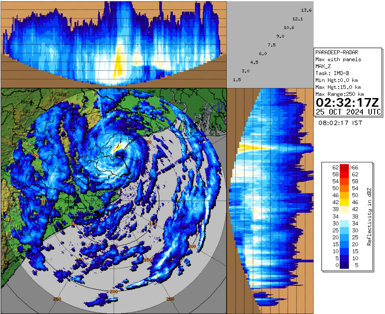
RADAR OBSERVATIONS (MAX_Z) OF DWR PARADIP
